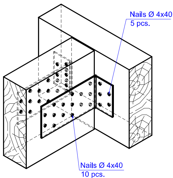
Figure D.45. Number and position of nails in the timber beam to timber beam connection with the angle brackets MKN 120 × 40 × 60 × 2,0
