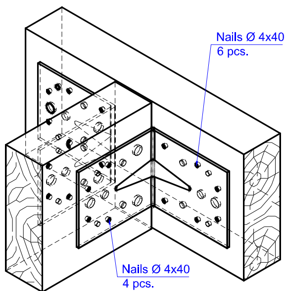
Figure D.39. Number and position of nails in the timber beam to timber beam connection with the angle brackets MKS 105 x 105 x 90 x 3,0
