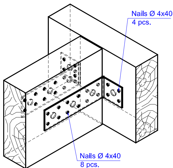
Figure D.51. Number and position of nails in the timber beam to timber beam connection with the angle brackets MKN 135 x 45 x 40 x 2,0 and MKN 135 x 45 x 40 x 2,5
