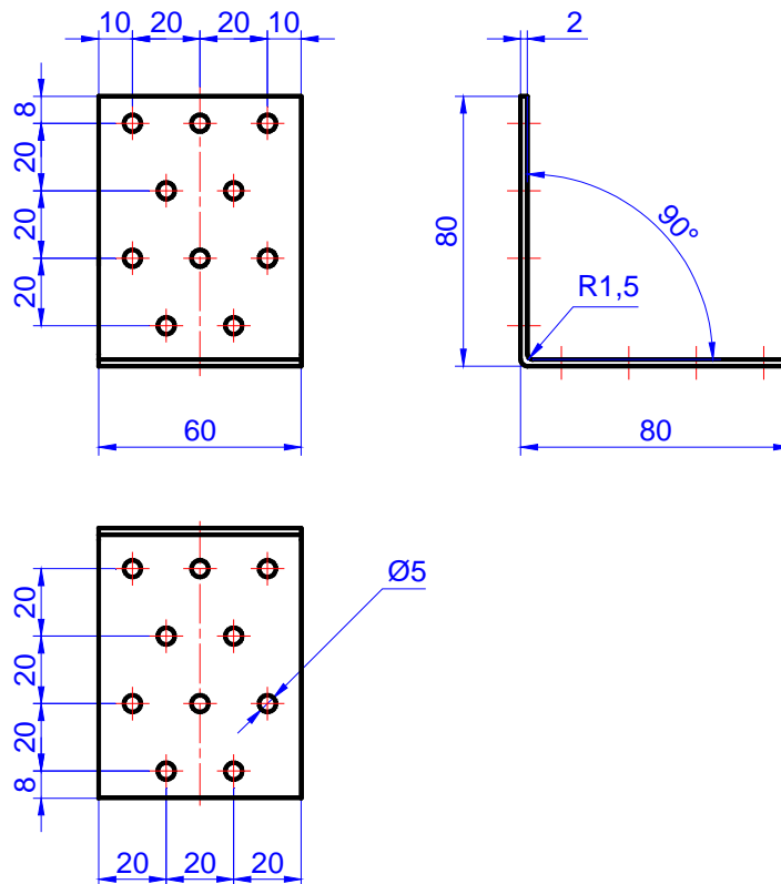
Figure C.3. Angle bracket MK 60 x 60 x 60 x 2,0
