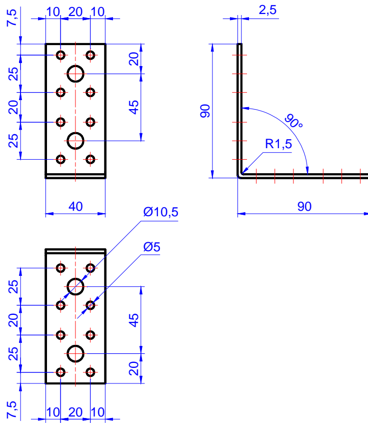
Figure C.31. Angle bracket MK 90 x 90 x 40 x 2,5
