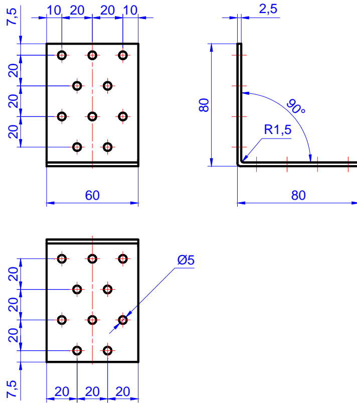
Figure C.15. Angle bracket MK 80 x 80 x 60 x 2,5
