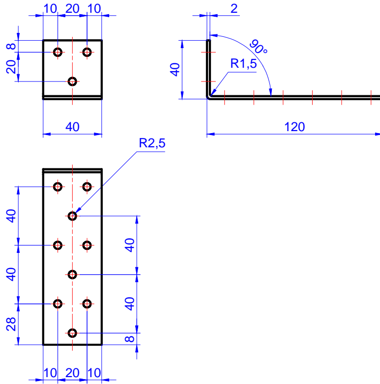
Figure C.60. Angle bracket MKN 120 x 40 x 40 x 2,0
