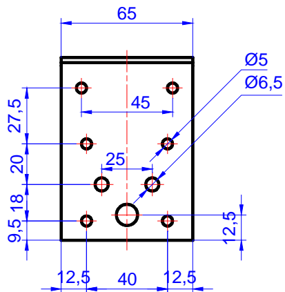
Figure C.34. Angle bracket MK 90 x 90 x 65 x 2,5
