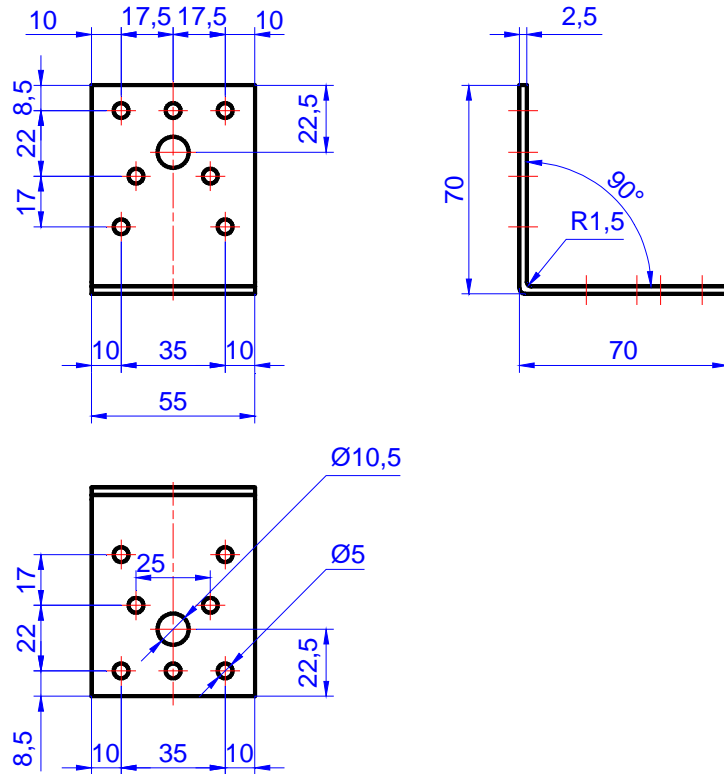
Figure C.29. Angle bracket MK 70 x 70 x 55 x 2,5
