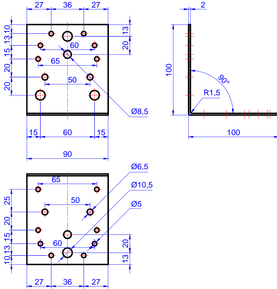
Figure C.35. Angle bracket MK 100 x 100 x 90 x 2,0
