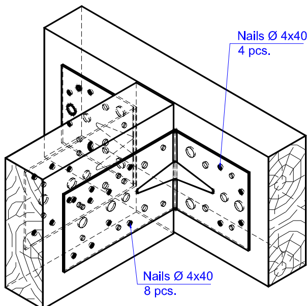
Figure D.42. Number and position of nails in the timber beam to timber beam connection with the angle brackets MKNS 150 x 100 x 90 x 2,0 and MKNS 150 x 100 x 90 x 2,5
