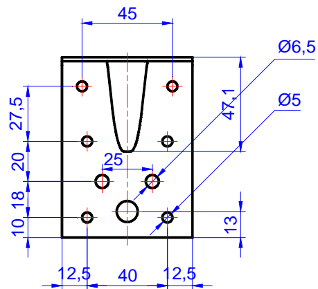
Figure C.49. Angle bracket MKS 90 x 90 x 65 x 2,0
