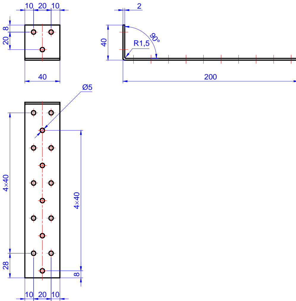
Figure C.65. Angle bracket MKN 200 x 40 x 40 x 2,0
