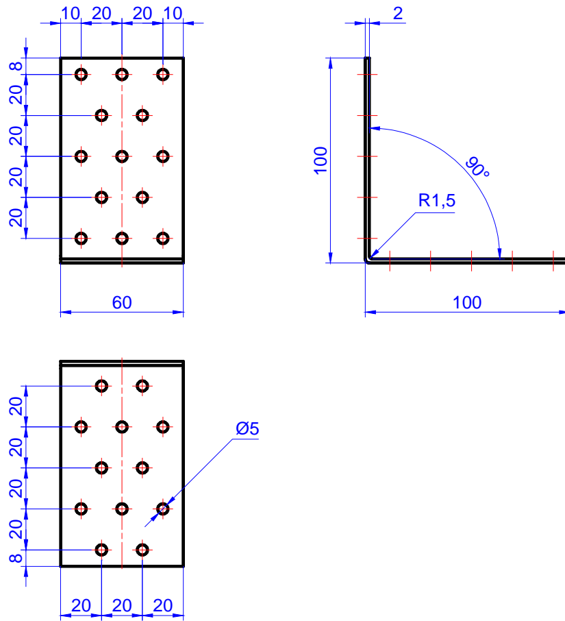
Figure C.5. Angle bracket MK 100 x 100 x 60 x 2,0
