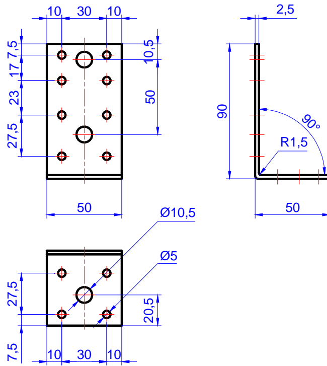
Figure C.67. Angle bracket MKN 90 x 50 x 50 x 2,5
