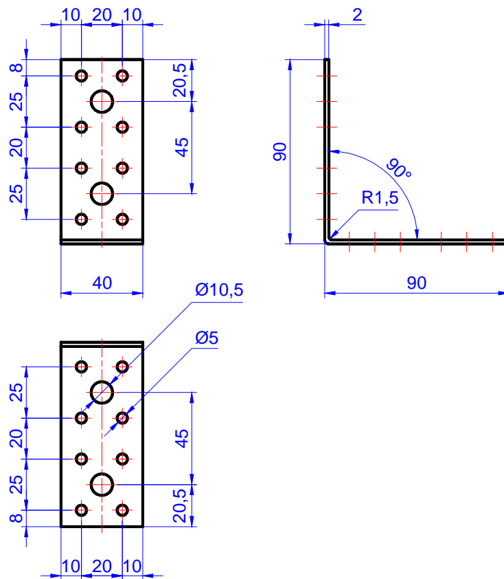
Figure C.30. Angle bracket MK 90 x 90 x 40 x 2,0
