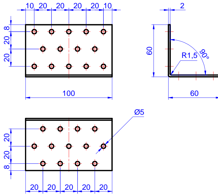
Figure C.9. Angle bracket MK 60 x 60 x 100 x 2,0
