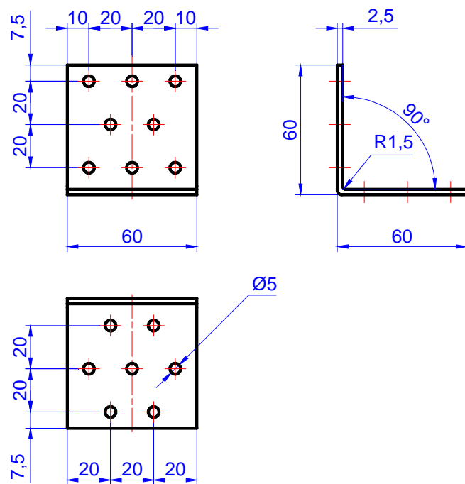
Figure C.14. Angle bracket MK 60 x 60 x 60 x 2,5
