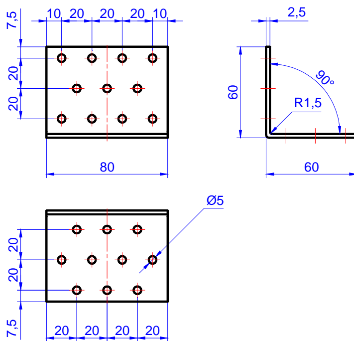
Figure C.17. Angle bracket MK 60 x 60 x 80 x 2,5
