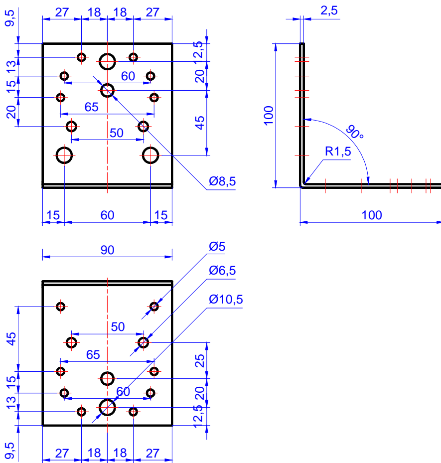
Figure C.36. Angle bracket MK 100 x 100 x 90 x 2,5
