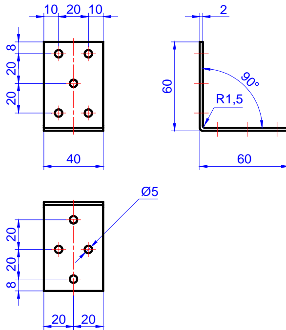
Figure C.1. Angle bracket MK 60 x 60 x 40 x 2,0
