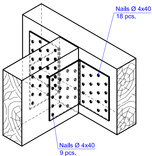
Figure D.10. Number and position of nails in the timber beam to timber beam connection with the angle brackets MK 80 × 80 × 100 × 2,0
