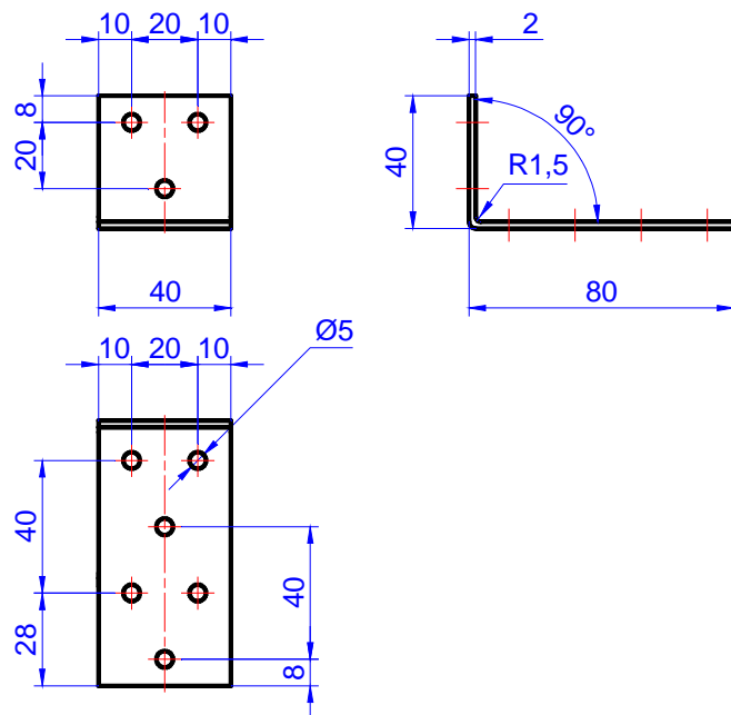
Figure C.61. Angle bracket MKN 80 x 40 x 40 x 2,0
