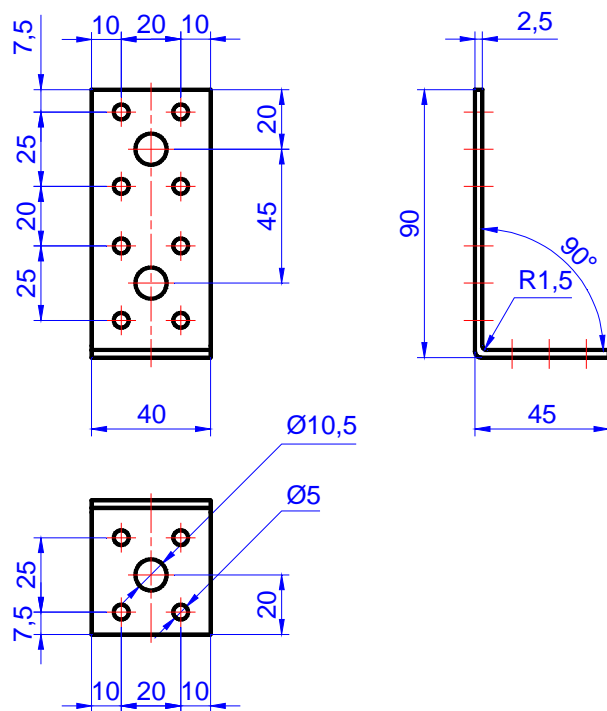
Figure C.68. Angle bracket MKN 95 x 45 x 40 x 2,5
