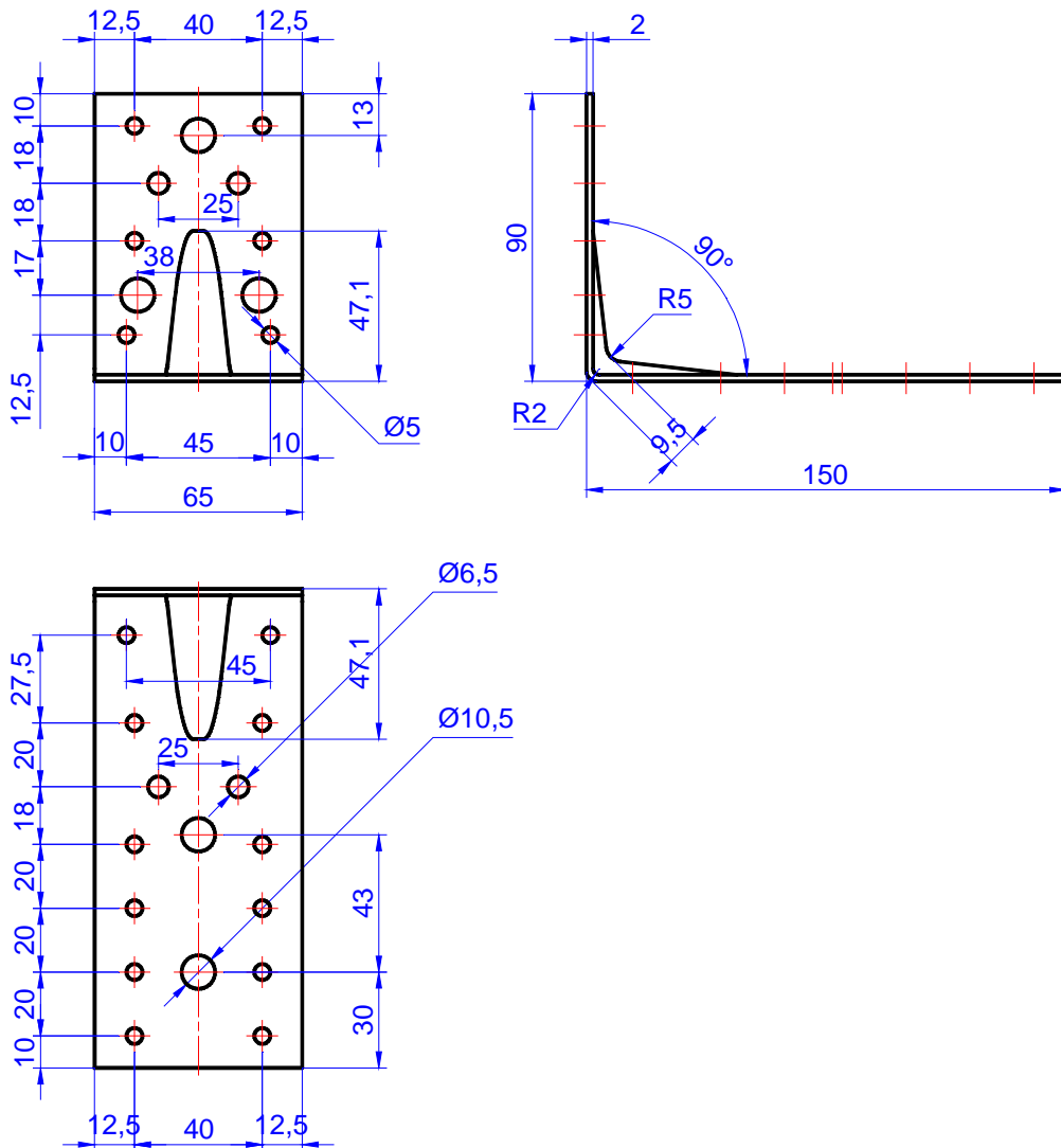
Figure C.56. Angle bracket MKNS 150 x 90 x 65 x 2,0
