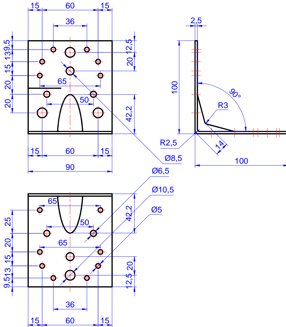
Figure C.52. Angle bracket MKS 100 x 100 x 90 x 2,5
