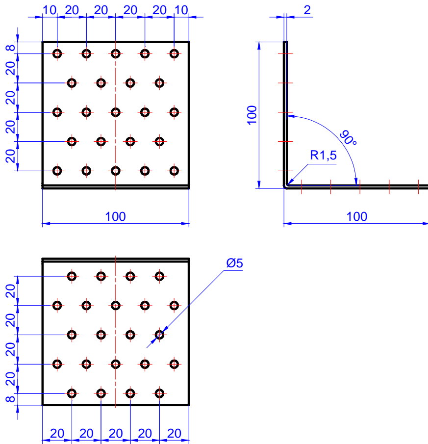
Figure C.1.1. Angle bracket MK 100 x 100 x 100 x 2,0
