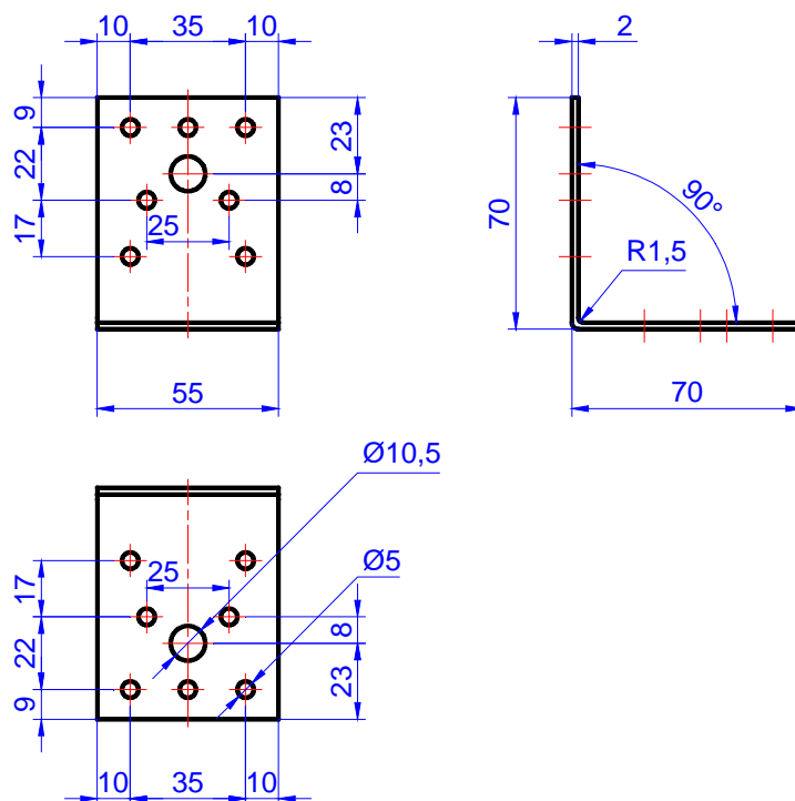
Figure C.28. Angle bracket MK 70 x 70 x 55 x 2,0
