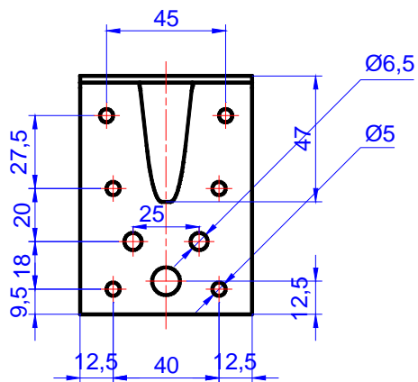
Figure C.50. Angle bracket MKS 90 x 90 x 65 x 2,5
