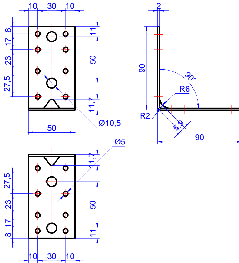
Figure C.47. Angle bracket MKS 90 x 90 x 50 x 2,0
