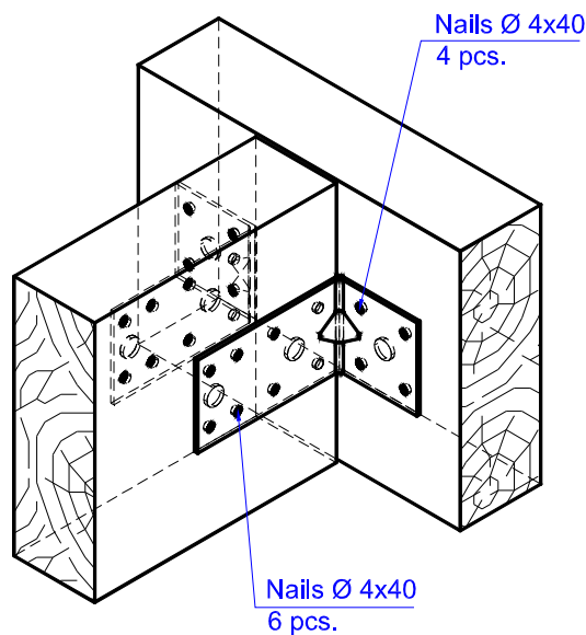
Figure D.40. Number and position of nails in the timber beam to timber beam connection with the angle brackets MKNS 90 x 50 x 50 x 2,0 and MKNS 90 x 50 x 50 x 2,5
