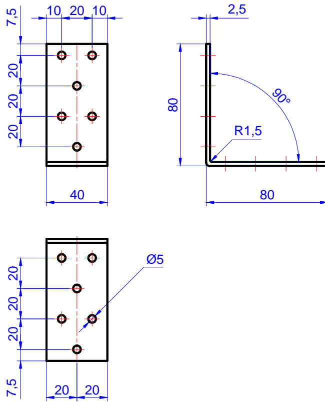
Figure C.13. Angle bracket MK 80 x 80 x 40 x 2,5
