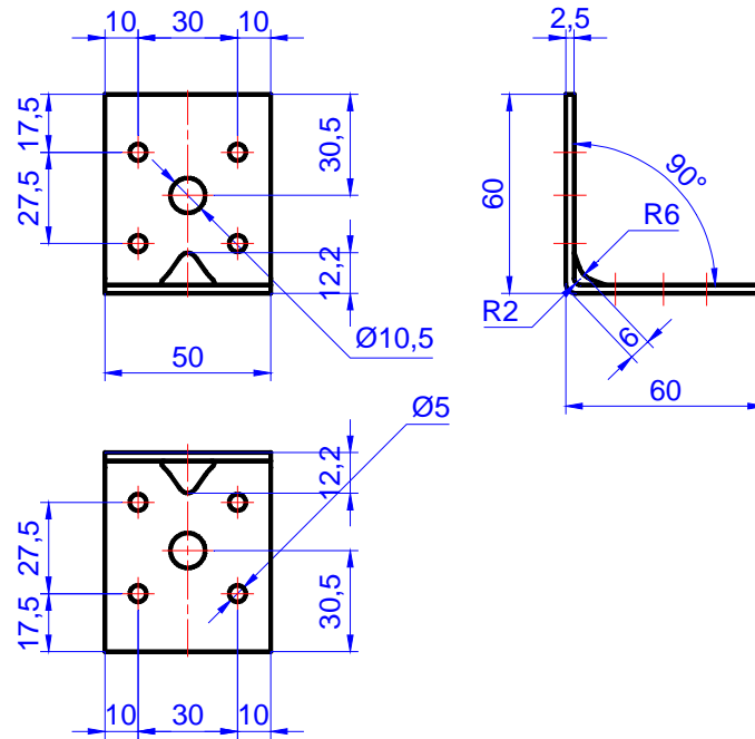
Figure C.43. Angle bracket MKS 60 × 60 × 50 × 2,5
