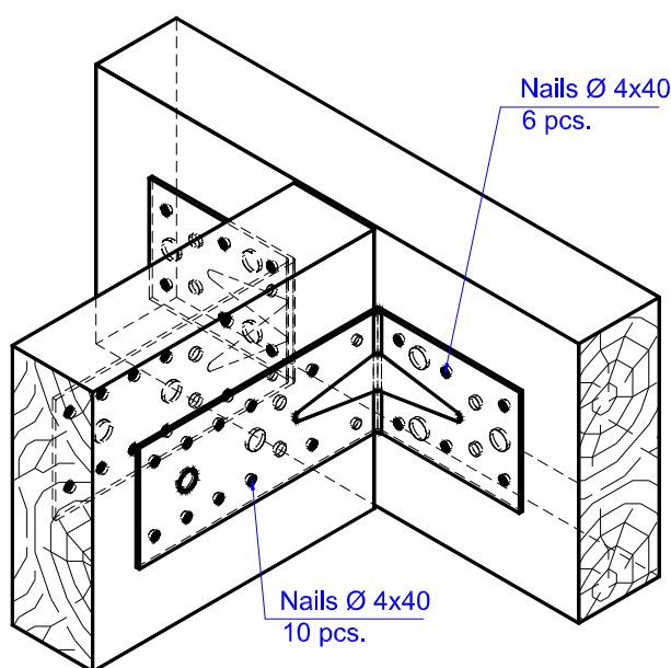
Figure D.41. Number and position of nails in the timber beam to timber beam connection with the angle brackets MKNS 150 x 90 x 65 x 2,0 and MKNS 150 x 90 x 65 x 2,5
