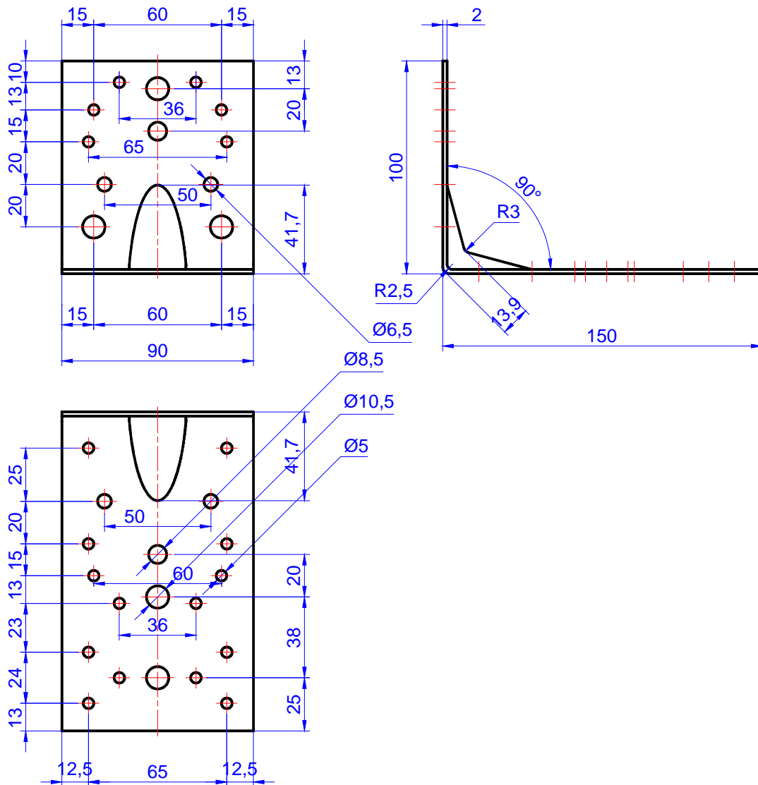
Figure C.58. Angle bracket MKNS 150 x 100 x 90 x 2,0
