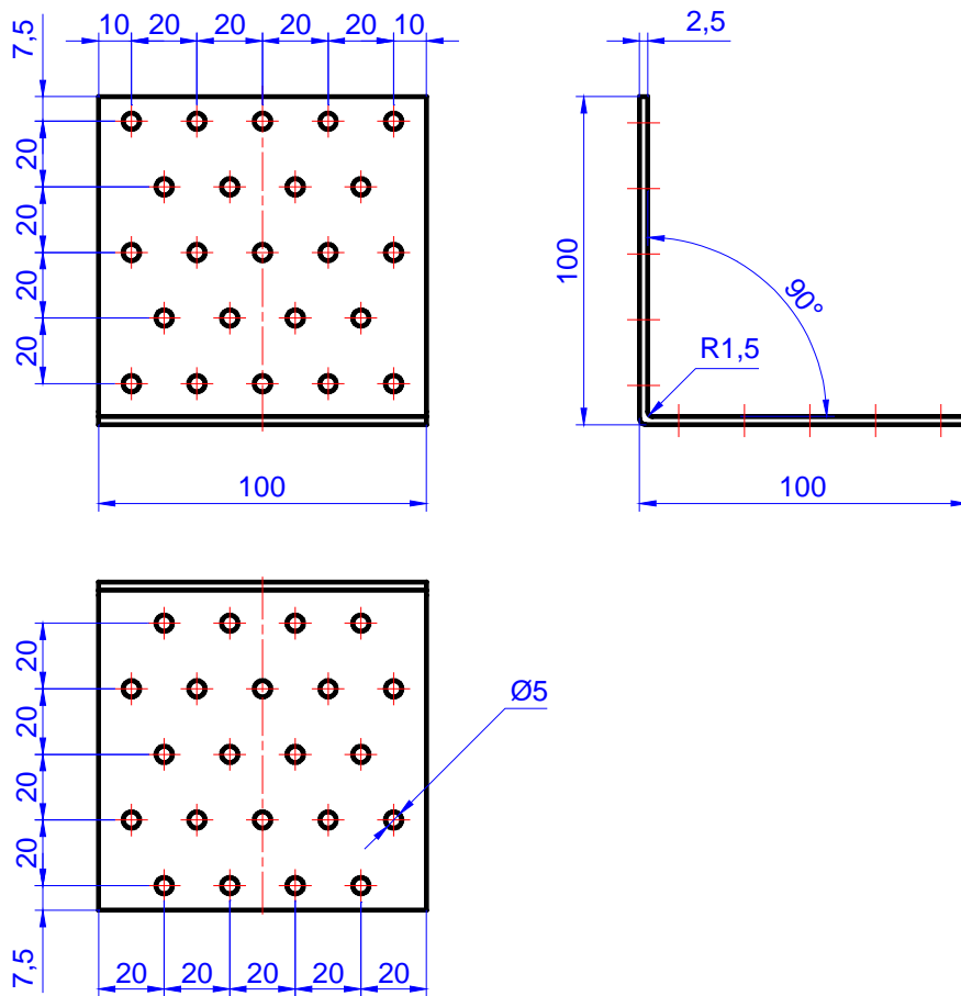
Figure C.22. Angle bracket MK 100 x 100 x 100 x 2,5
