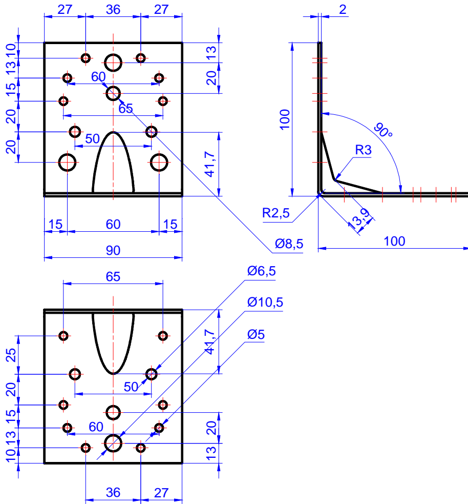
Figure C.51. Angle bracket MKS 100 x 100 x 90 x 2,0
