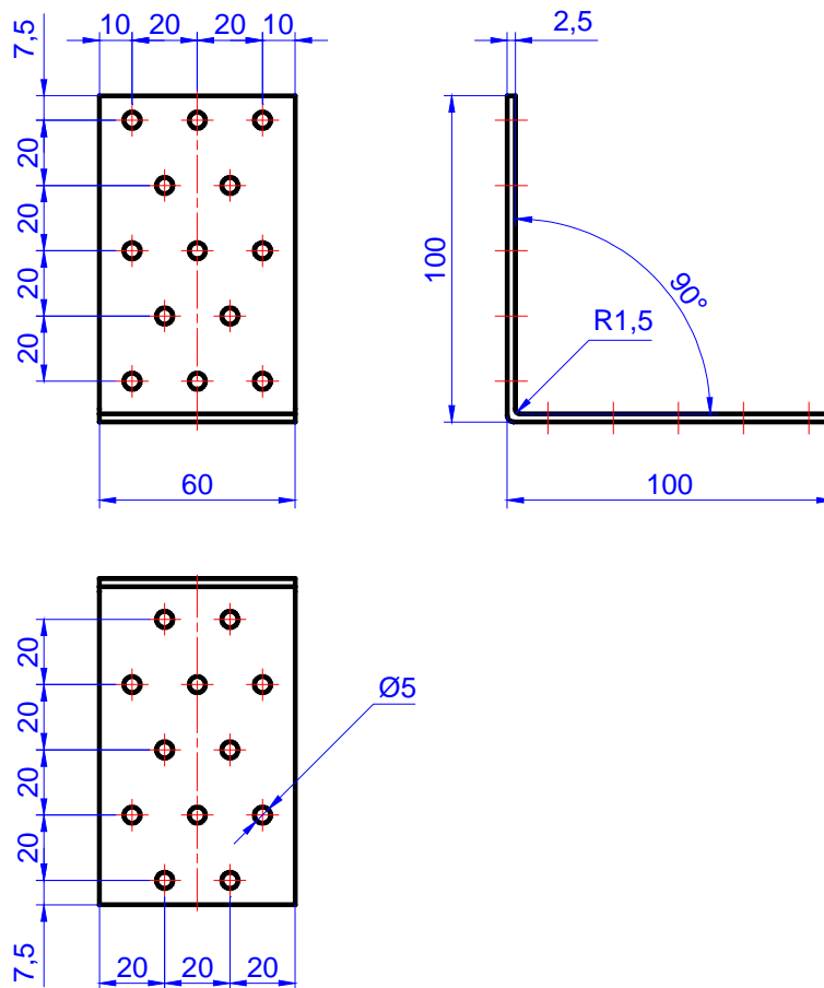
Figure C.16. Angle bracket MK 100 x 100 x 60 x 2,5
