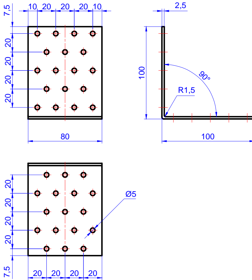
Figure C.19. Angle bracket MK 100 x 100 x 80 x 2,5
