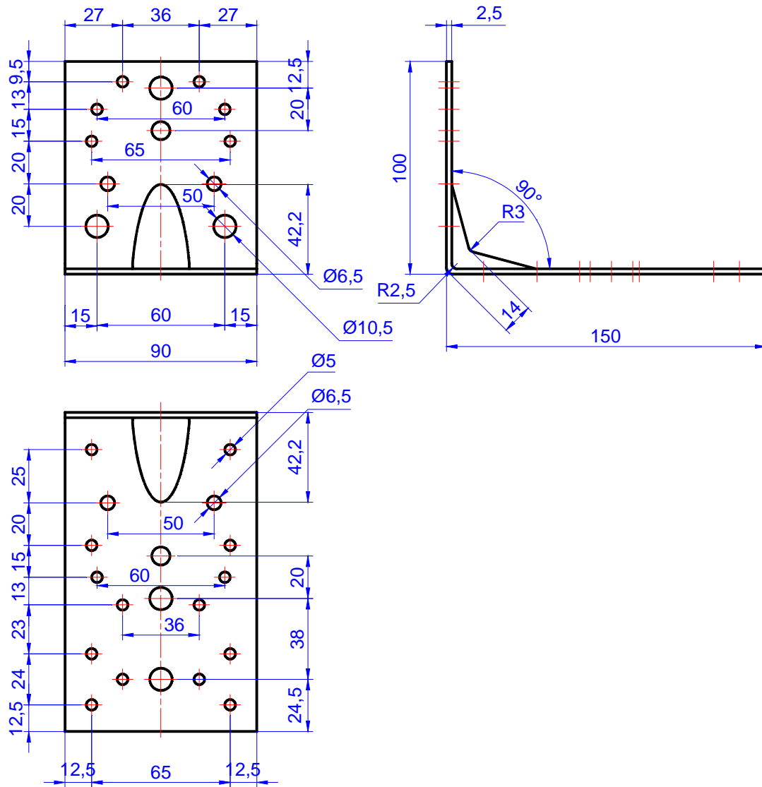
Figure C.59. Angle bracket MKNS 150 x 100 x 90 x 2,5
