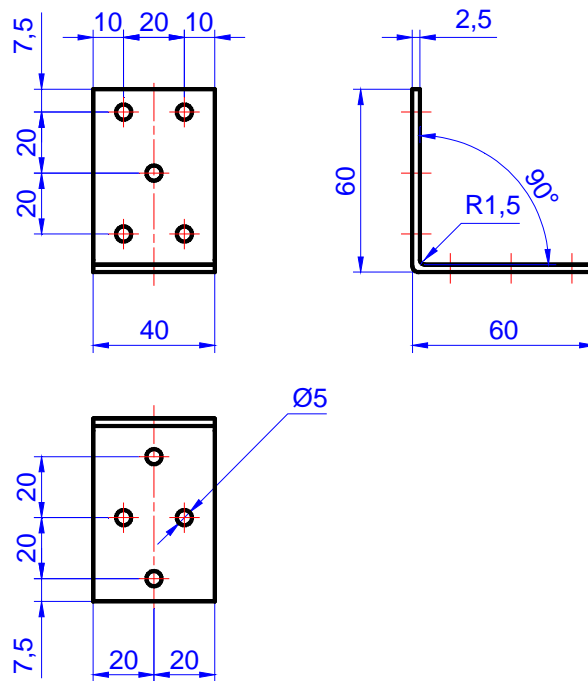
Figure C.12. Angle bracket MK 60 x 60 x 40 x 2,5
