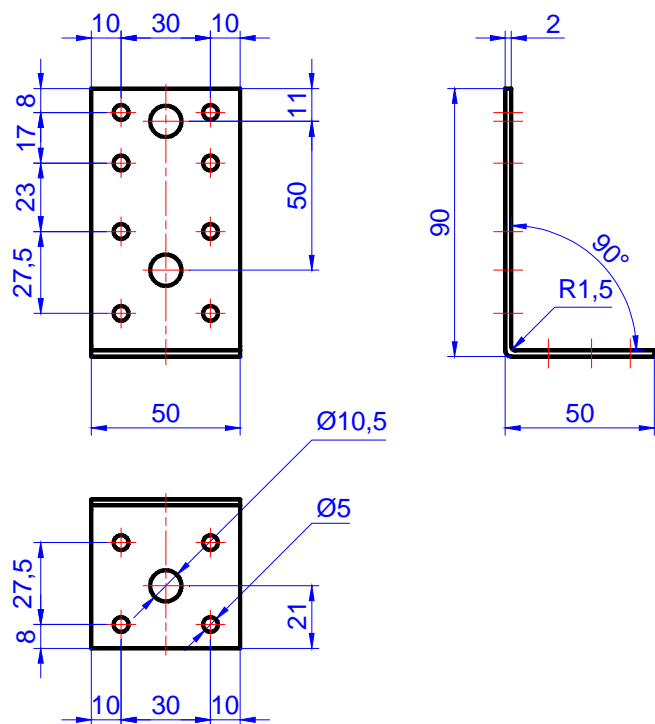
Figure C.66. Angle bracket MKN 90 x 50 x 50 x 2,0
