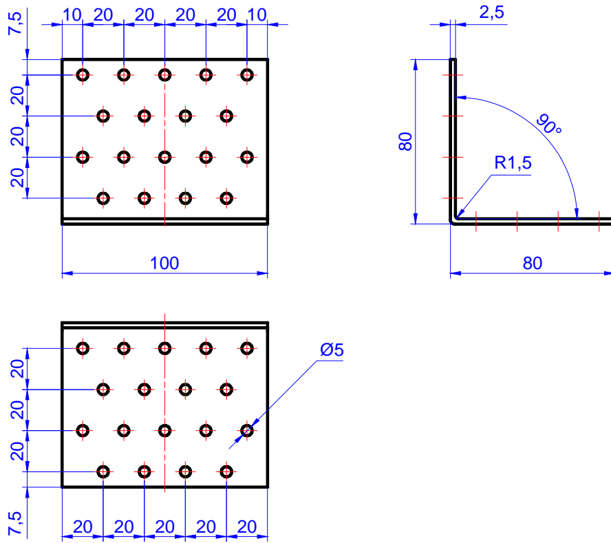
Figure C.21. Angle bracket MK 80 x 80 x 100 x 2,5
