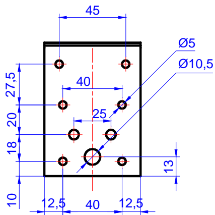
Figure C.33. Angle bracket MK 90 x 90 x 65 x 2,0
