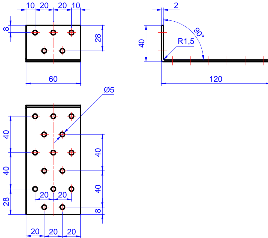
Figure C.62. Angle bracket MKN 120 x 40 x 60 x 2,0
