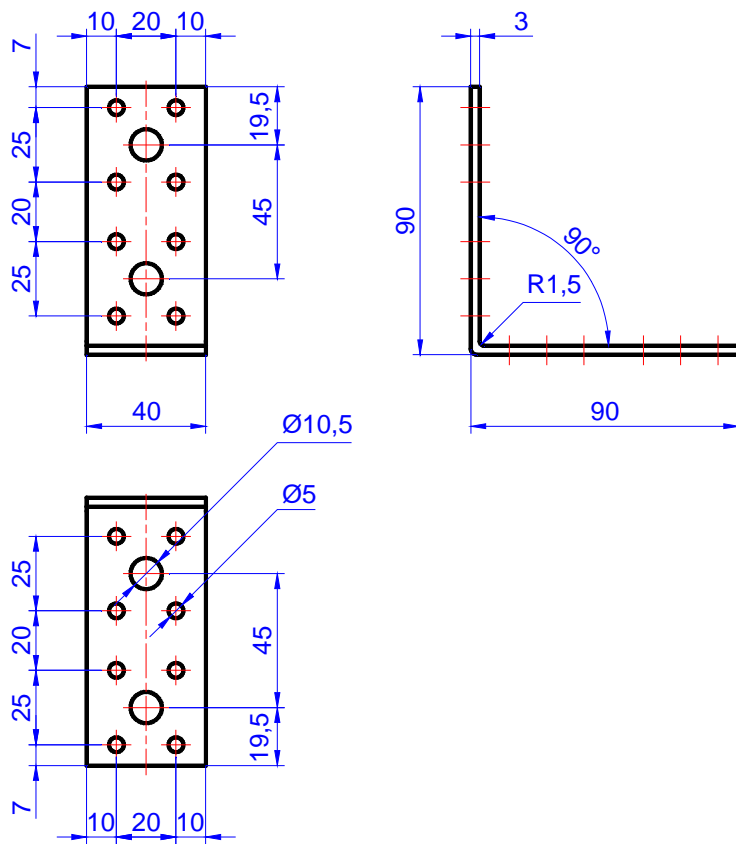
Figure C.32. Angle bracket MK 90x90x40x3,0
