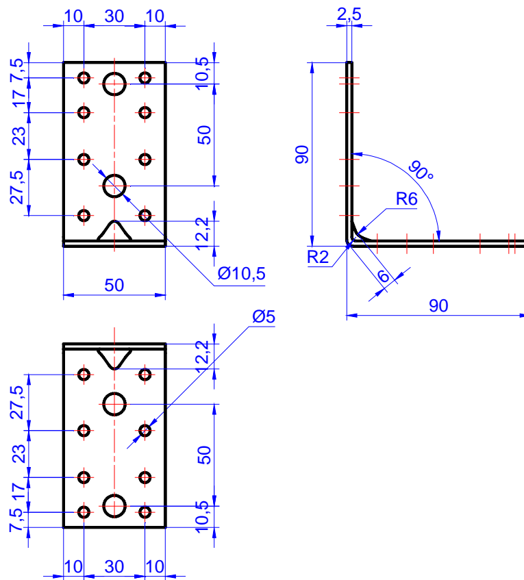
Figure C.48. Angle bracket MKS 90 x 90 x 50 x 2,5
