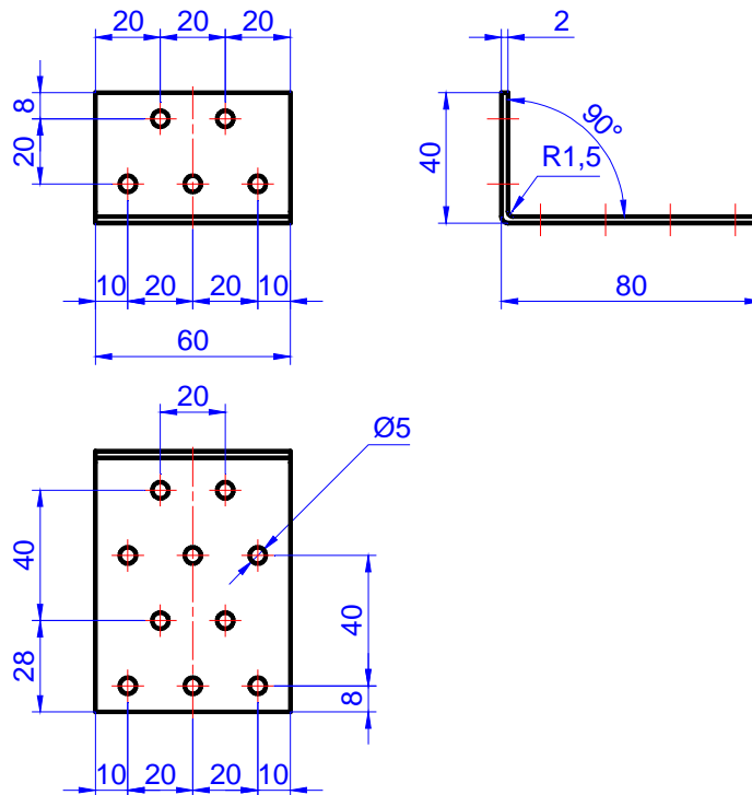
Figure C.63. Angle bracket MKN 80 x 40 x 60 x 2,0
