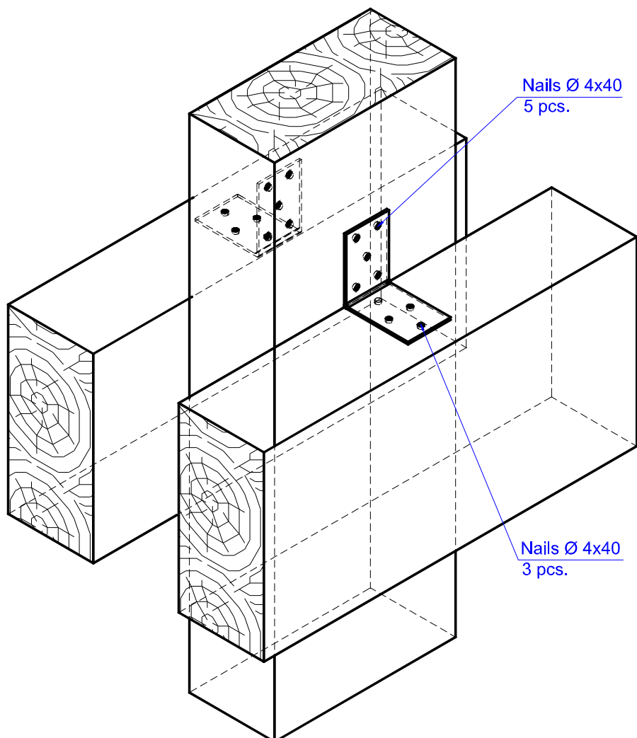
Figure D.52. Number and position of nails in the timber beam to timber column connection with the angle brackets MK 60 x 60 x 40 x 2,0
