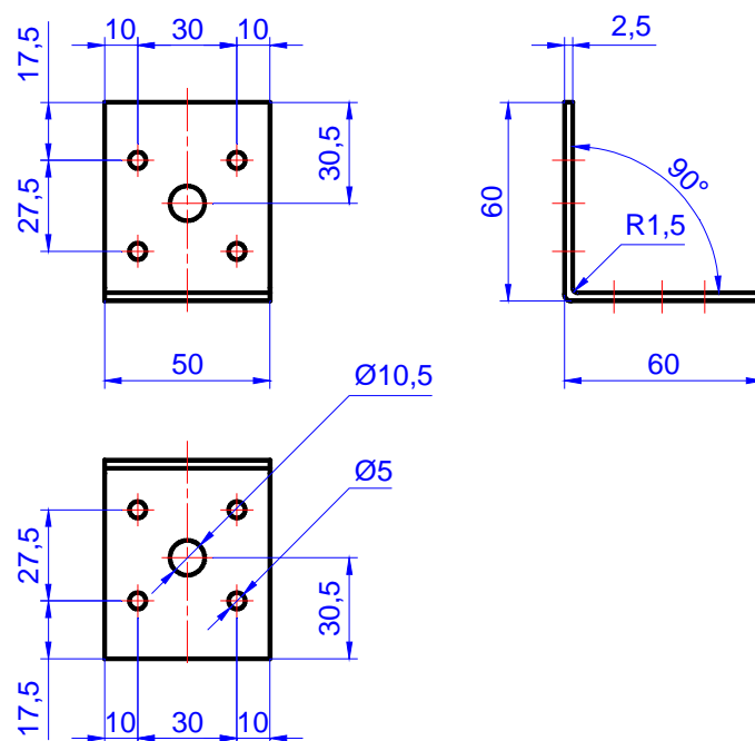
Figure C.27. Angle bracket MK 60 x 60 x 50 x 2,5
