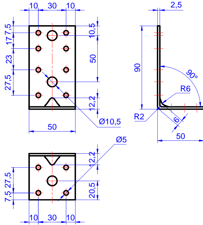
Figure C.55. Angle bracket MKNS90 x 50 x 50 x 2,5
