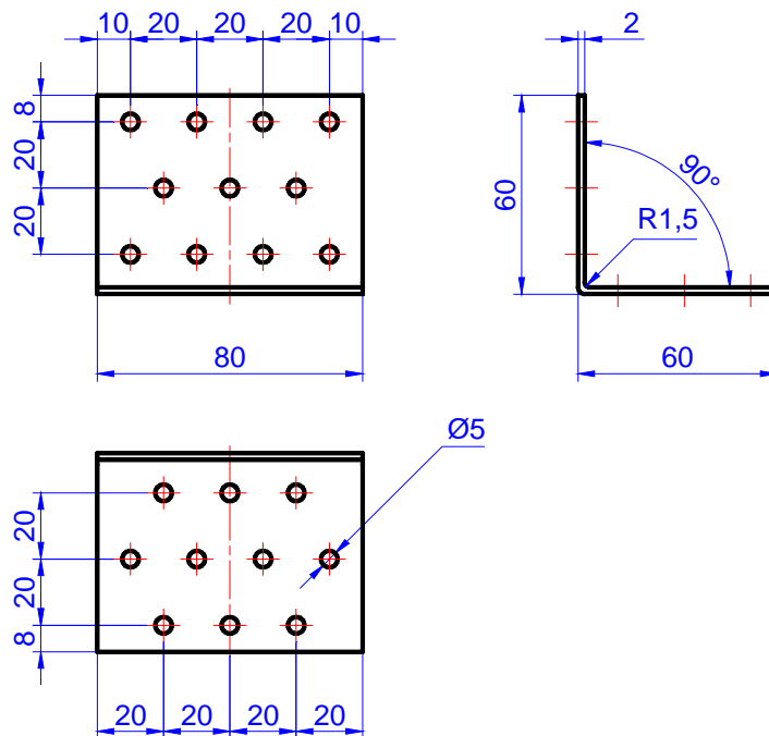
Figure C.6. Angle bracket MK 60 x 60 x 80 x 2,0
