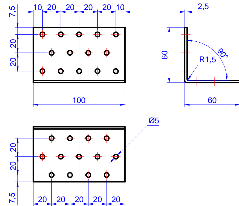
Figure C.20. Angle bracket MK 60 x 60 x 100 x 2,5
